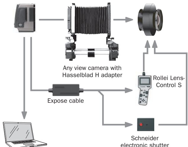
Host computer with FireWire, running Pocus
