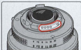
CPU contacts of CPU Nikkor lens
