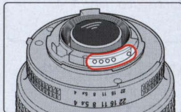
CPU contacts of CPU Nikon lens
