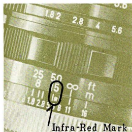
Infra-Red Mark
